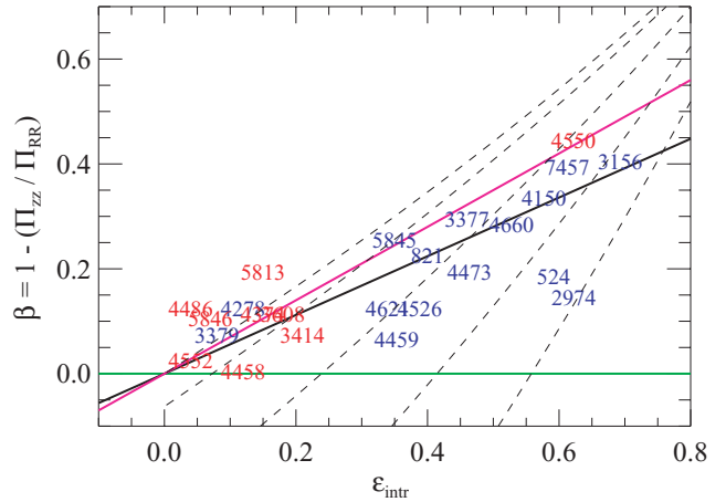
Figure 7. Anisotropy parameter \beta in the meridional plane versus the average intrinsic ellipticity \epsilon_{\text{intr}} of the galaxies. The observed anisotropy is related to the intrinsic ellipticity of the galaxies. The thick black solid line is the best-fitting relation. The dashed lines show the predictions of the tensor virial equations, in the form of equation (14), for different values of the V/\sigma = 0, 0.25, \dots, 1 (see text for details). The red and blue labels refer to the slow and fast rotators, respectively. The magenta line shows the same relation \beta = 0.7\epsilon_{\text{intr}} as the one in Fig. 9, while the green line indicates isotropy.
