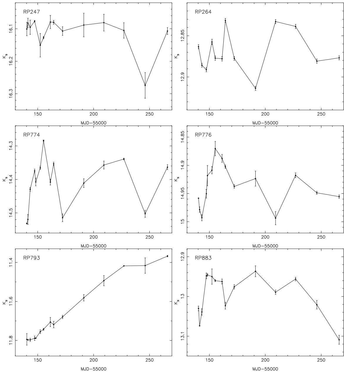
Fig. 3. VMC K_s lightcurves of the variables in Tab. 5. Observations taken on the same night were combined using a weighted mean.
