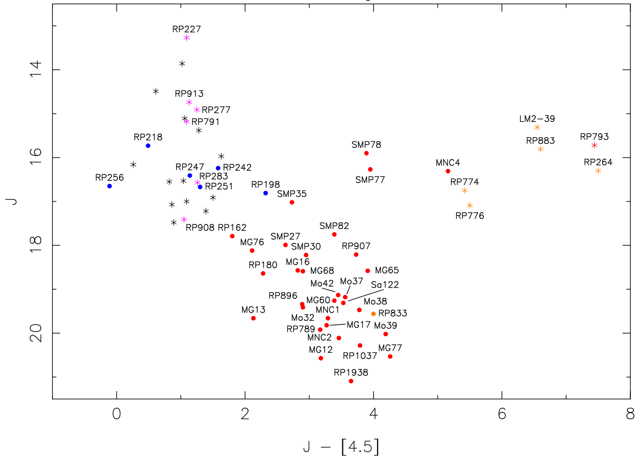
Fig. 7. As in Fig. 6 but for U - B vs. J - K_s (top) and J vs. J - [4.5] (bottom).
