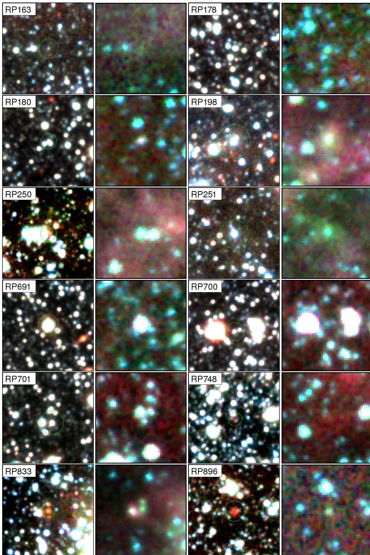
Fig. B.13. Figure B.12 (continued).
