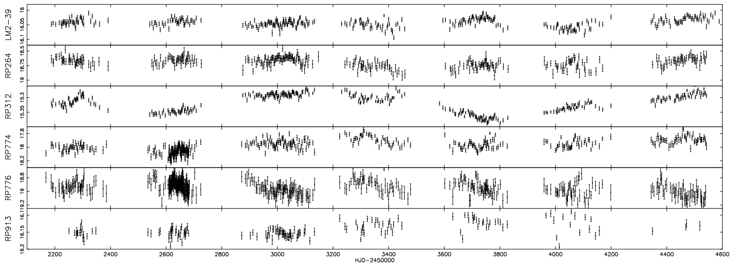
Fig. 4. OGLE-III I -band lightcurves for a sample of non-periodic variables.
