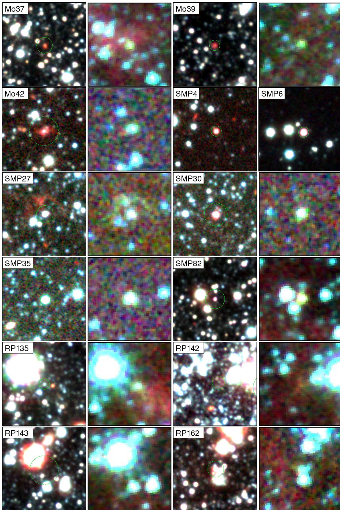
Fig. B.12. Figure B.11 (continued).
