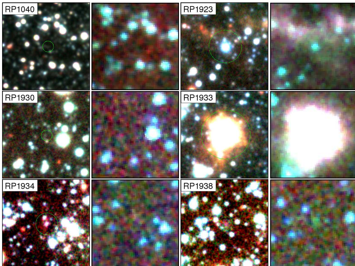
Fig. B.14. Figure B.13 (continued).
