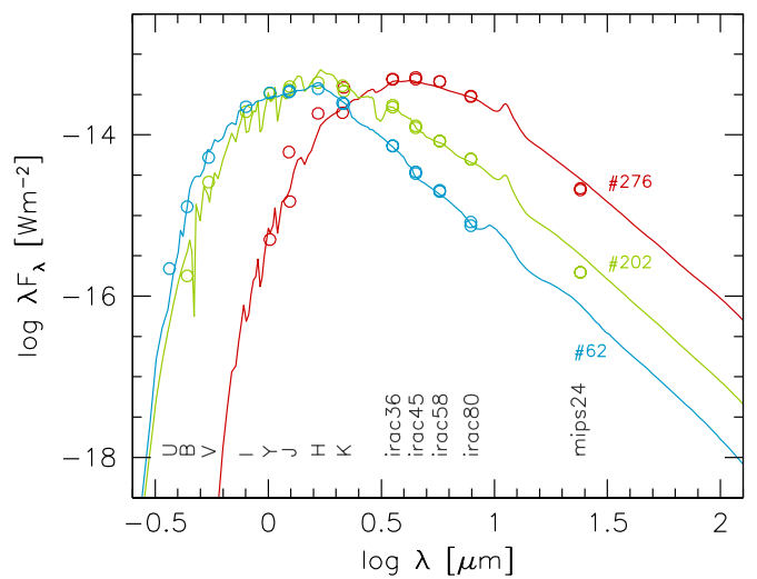
Fig. 2: Photometric data points ( open circles ) and the fitted SEDs ( lines ) for three AGB stars: a blue O-rich star ( J - K_s = 1.2 mag, id 62), and two C-rich stars ( J - K_s = 1.5 mag, id 202; and J - K_s \sim 4 mag, id 276).
