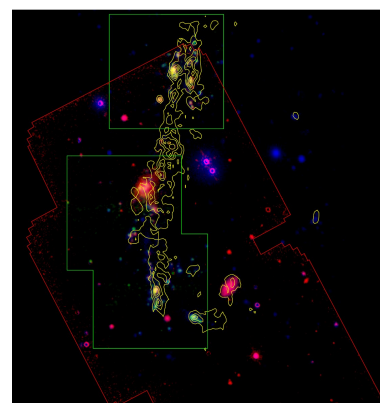
NGC 5291, a spectacular interacting system having many intergalactic star forming regions seen in ultraviolet (blue), ionized hydrogen (green), infrared (red) and gas (yellow contours)
